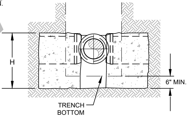
SECTION TEE
