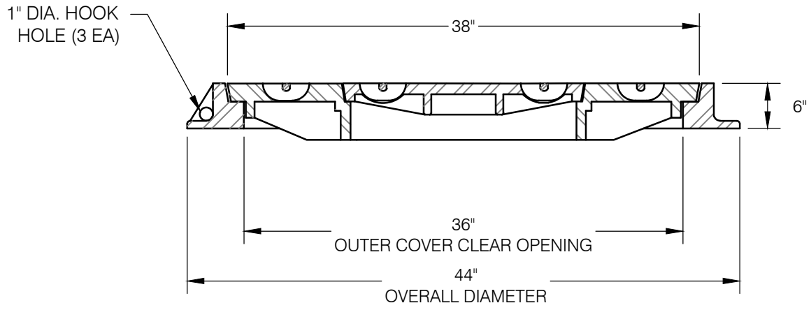
SECTION A
