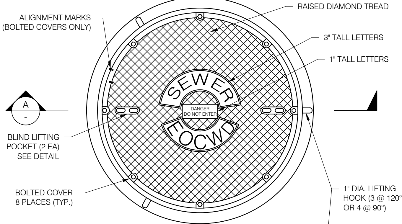
PLAN
