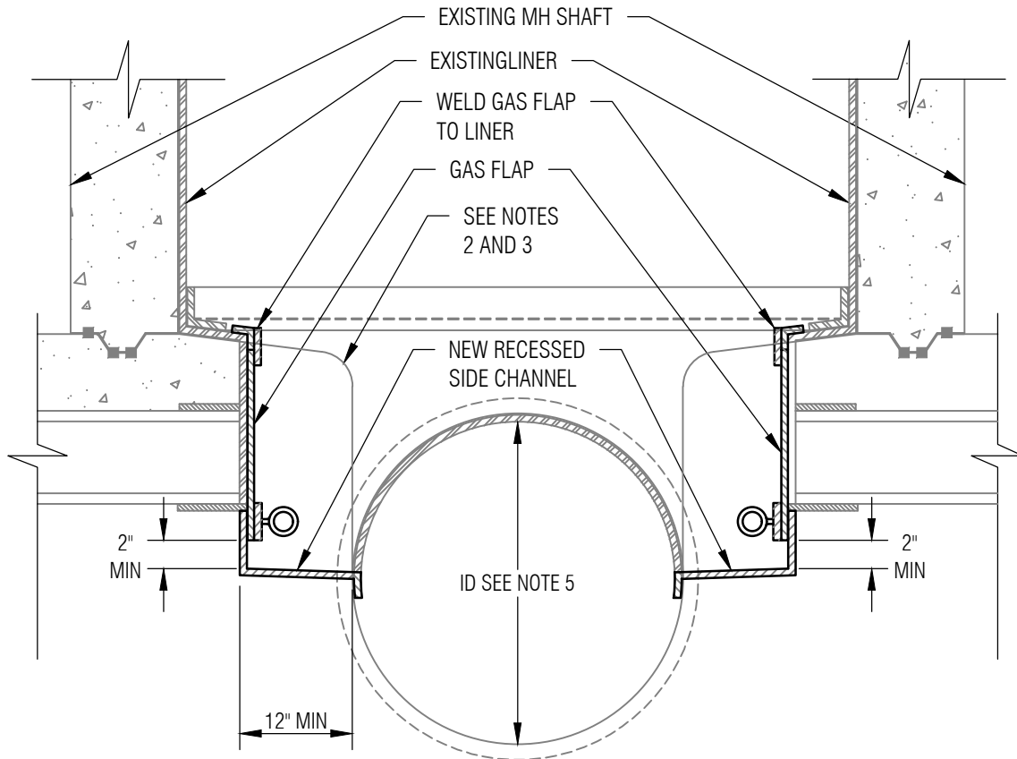
SECTION A
