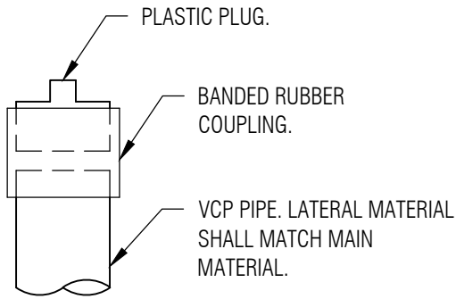
VCP STOPPER DETAIL DETAIL 2
