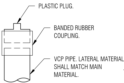
VCP STOPPER DETAIL DETAIL 2
