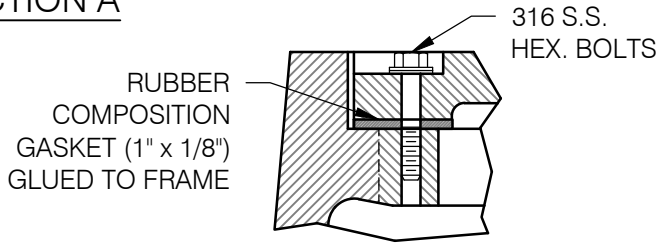
BOLTING/Self-SEAL DETAIL
