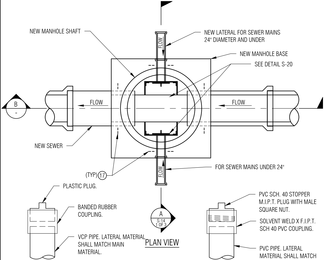
VCP STOPPER DETAIL DETAIL 2
