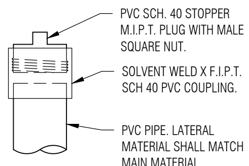
PVC STOPPER DETAIL DETAIL 3
