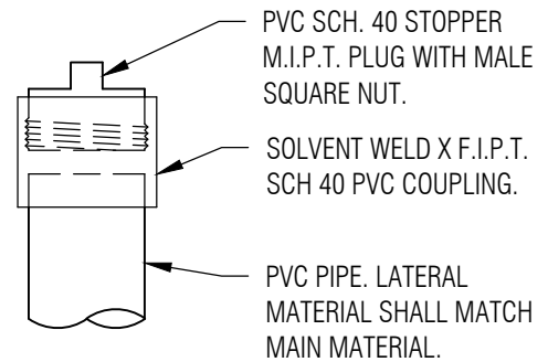
PVC STOPPER DETAIL DETAIL 3
