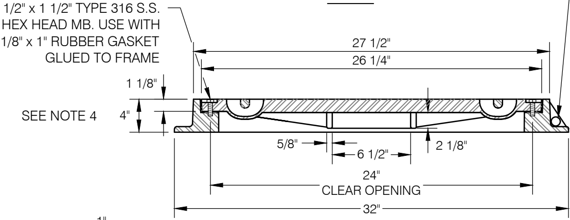
SECTION A
