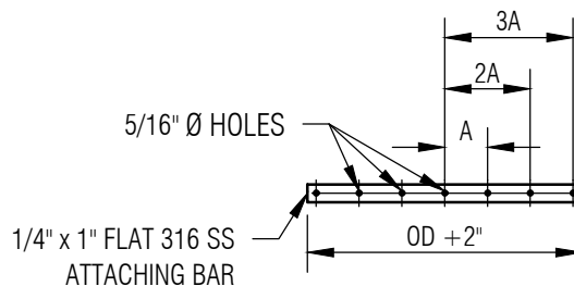
DETAIL 3 ATTACHING BAR SEE NOTE 2
